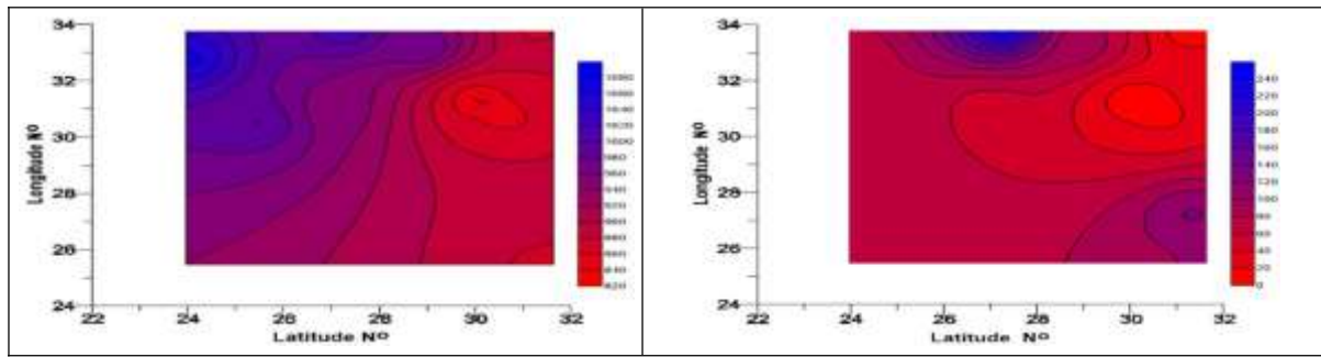
Figure 8: Annual mean of wind speed (km/h) at different locations over Egypt.
