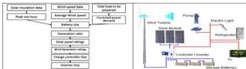
Figure 3: Flow chart of hybrid solar- wind resource
