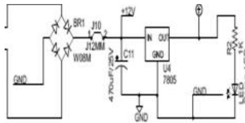
Figure 5: Circuit
