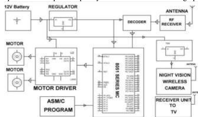
Figure 4: Receiver
