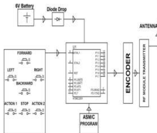
Figure 3: Transmitter Module
