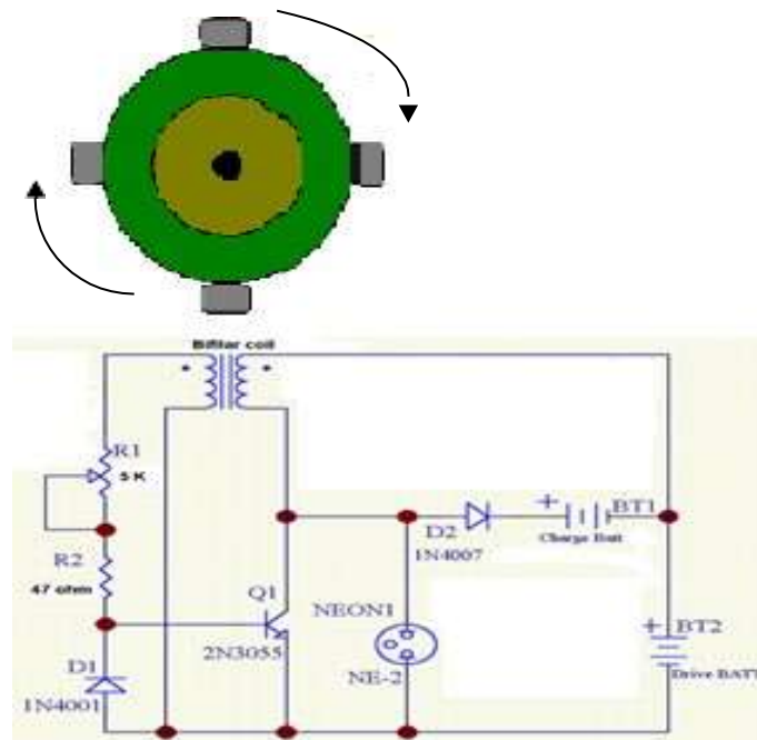
Figure 8: Schematic Circuit of Bedini SSG
