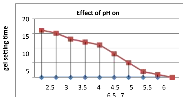
Figure. 1.2 Plot of pH against gel setting time in days
