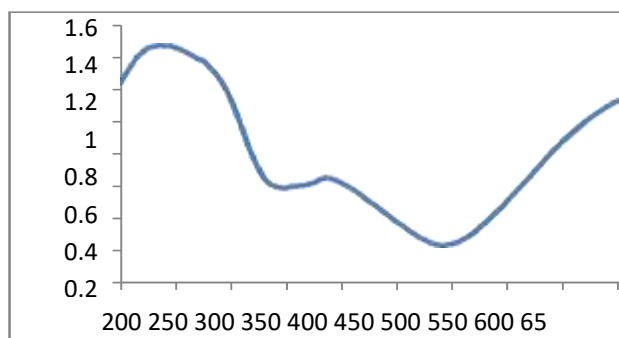
Figure 1.7 UV-VIS Spectra of copper Sulphide
