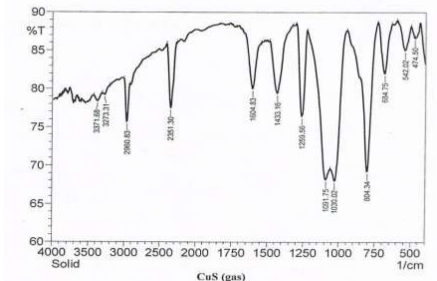
Figure 1.6 FT-IR spectrum of copper sulphide.
