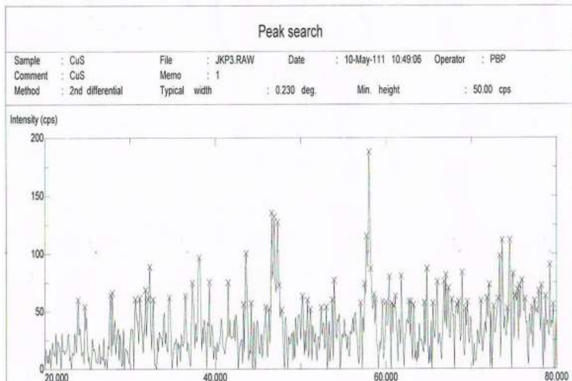
Figure 1.5 X-ray Diffractogram of copper sulphide
