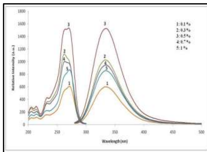
Fig. 2: Photoluminescence emission and excitation spectra.
