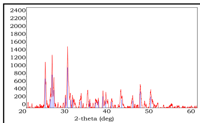
Fig. 1. XRD pattern of \text{CaB}_4\text{O}_7
