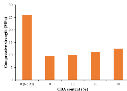
Fig. 5. Compressive strength of concrete mixes comprising CBA [33].
