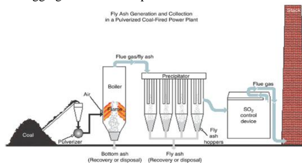
Fig. 1. Producing coal bottom ash in thermal power plants [31].
