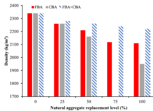
Fig. 4. The effect of CBA on the density [32].
